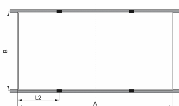
Clamp installation without cross beam (B3) Clamp size \geq 50\text{mm}
