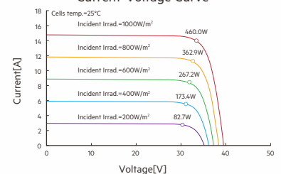
Current-Voltage Curve
