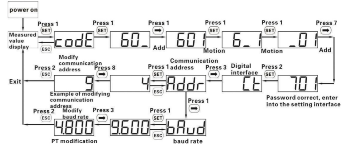
Diagram 3 Setting examples for modifying communication address and baud rate
