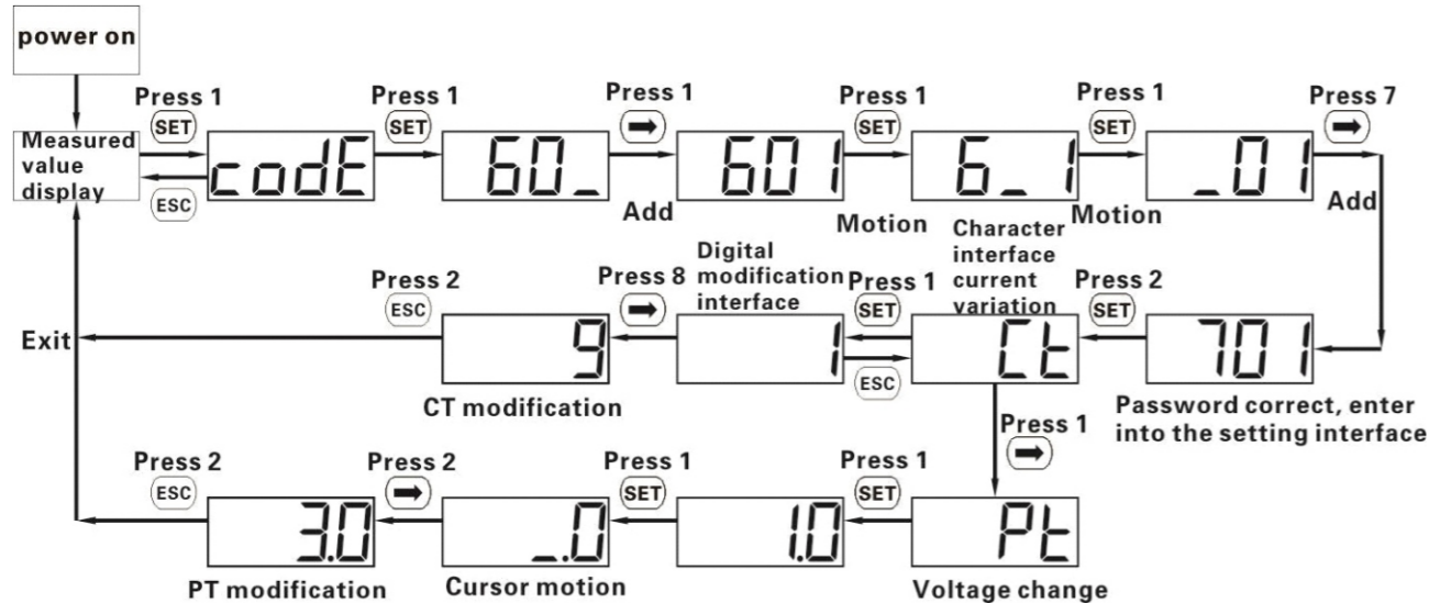
Diagram 2 Setting examples for modifying current ratio
