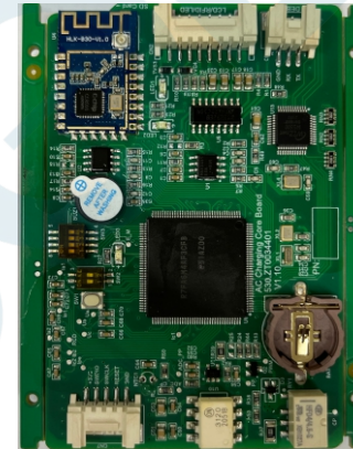
Micro SD slot of 22kW charger
